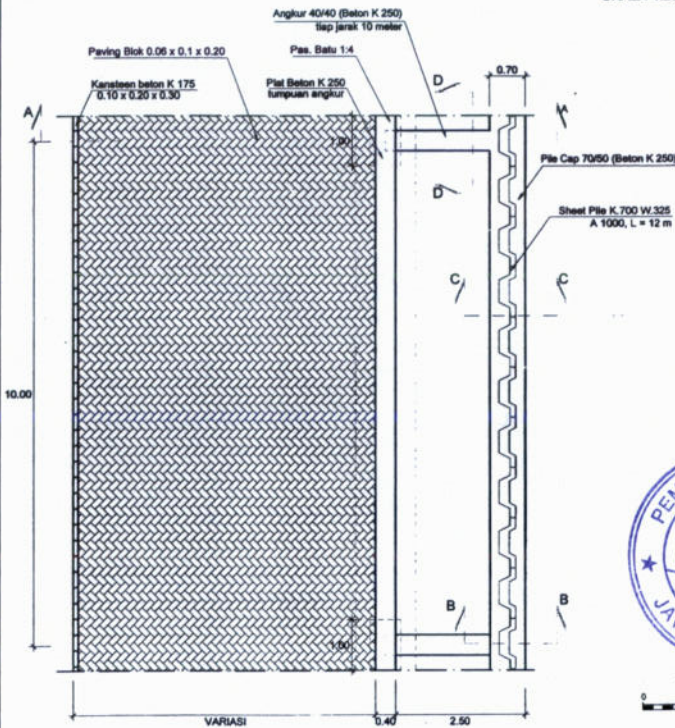
DENAH PASANGAN SHEET PILE SKALA 1:50
